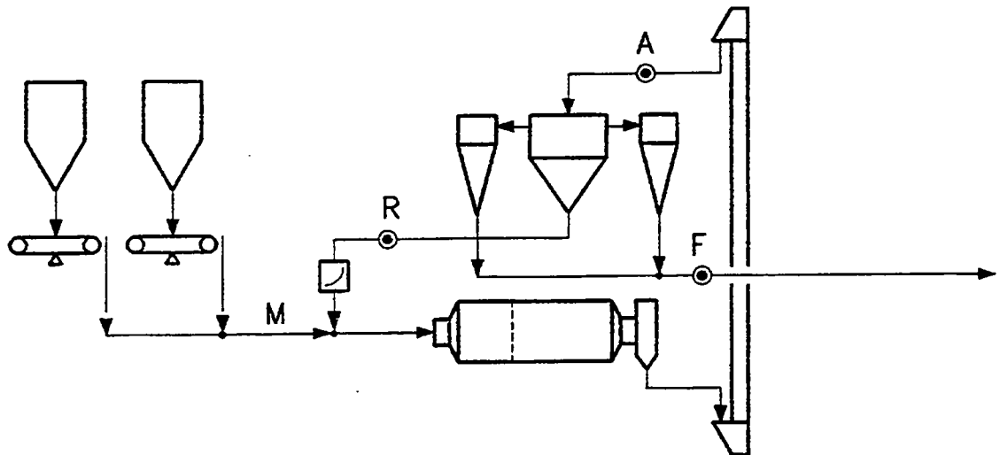
Figure 12 Sampling Points - Cyclone Air Separator
